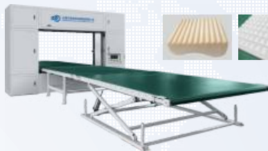
SR-CNC05 双环刀异形海绵数控切割机 (横刀+竖刀) Double CNC Circular Contour Cutting Machine (Horizontal and Vertical)
